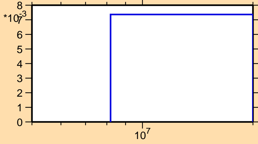
\sigma vs. E for ^{100}\text{Ru}(n,np)
