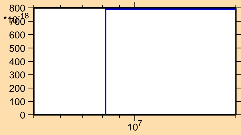
\sigma vs. E for ^{100}\text{Ru} (mt 45)
