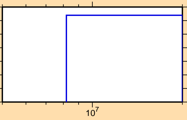
\sigma vs. E for ^{100}\text{Ru}(n,pd)
