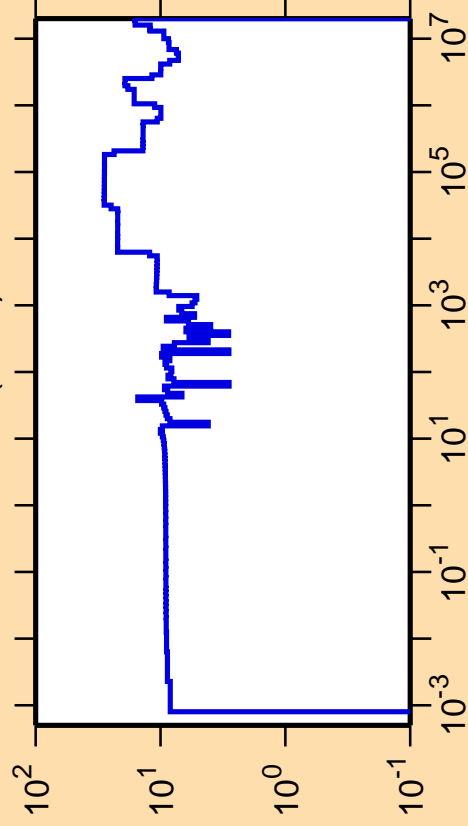
\Delta\sigma/\sigma vs. E for ^{101}\text{Ru}(n,\text{el.})
