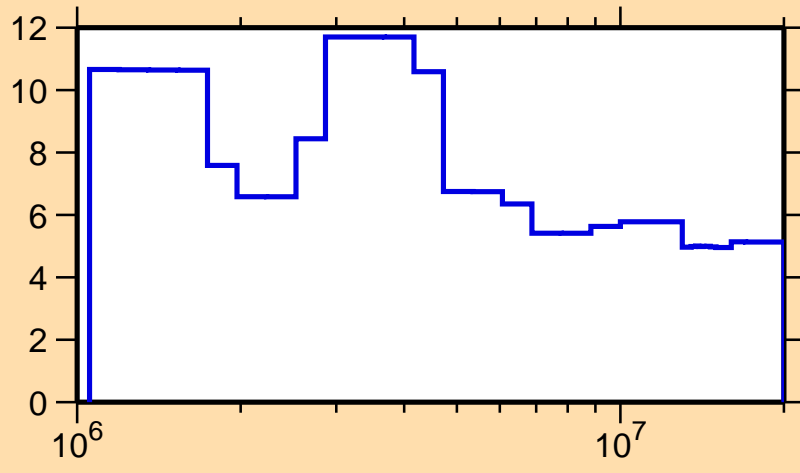
\Delta\sigma/\sigma vs. E for ^{101}\text{Ru}(n,n\text{onel.})
