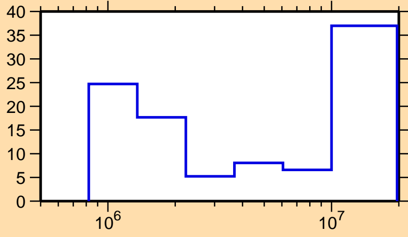
\Delta\sigma/\sigma vs. E for ^{101}\text{Ru}(n,n\text{cont.})
