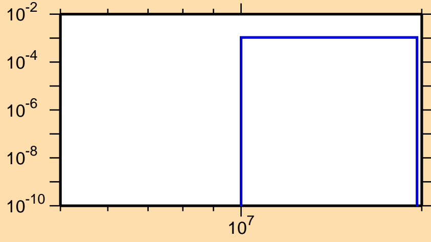
\sigma vs. E for ^{101}\text{Ru}(n,d)
