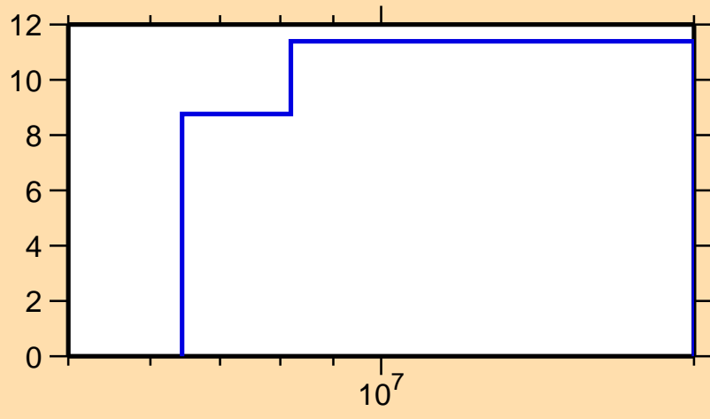
\Delta\sigma/\sigma vs. E for ^{101}\text{Ru}(n,2n)
