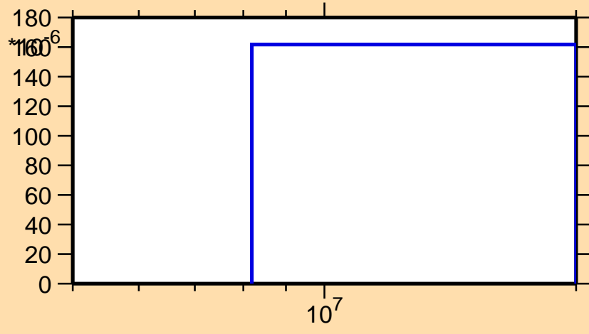
\sigma vs. E for ^{101}\text{Ru}(n,t)
