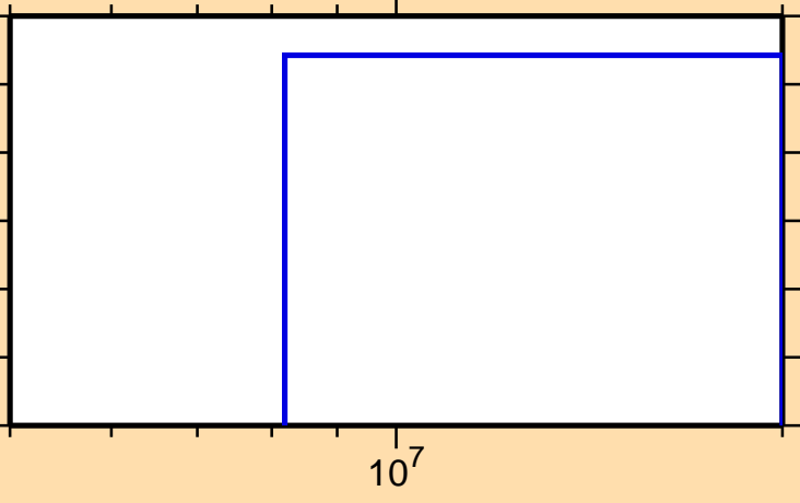
\sigma vs. E for ^{101}\text{Ru}(n,nd)
