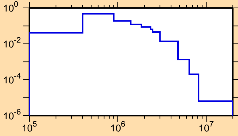
\sigma vs. E for ^{101}\text{Ru}(n,n_2)
