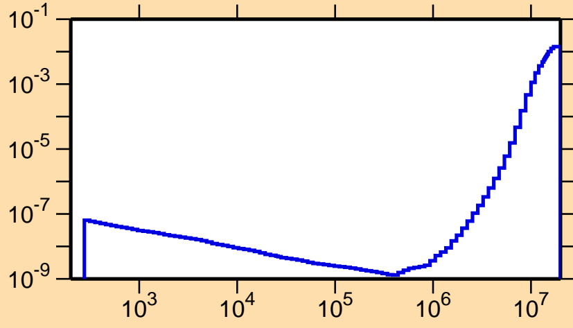
\sigma vs. E for ^{103}\text{Ru}(n,\alpha)
