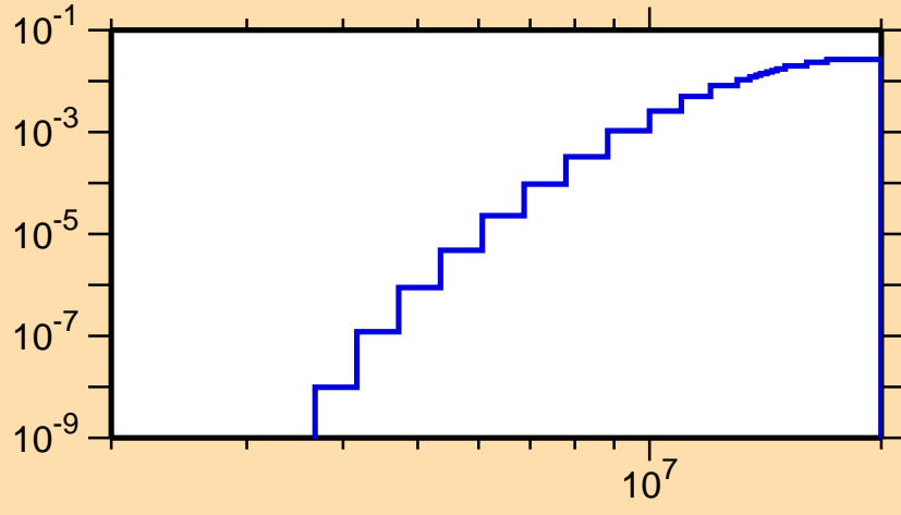
\sigma vs. E for ^{103}\text{Ru}(n,p)
