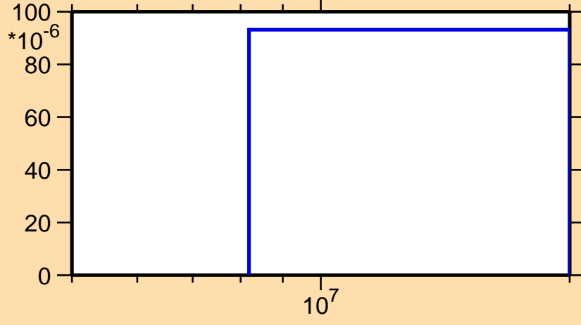
\sigma vs. E for ^{103}\text{Ru}(n,t)
