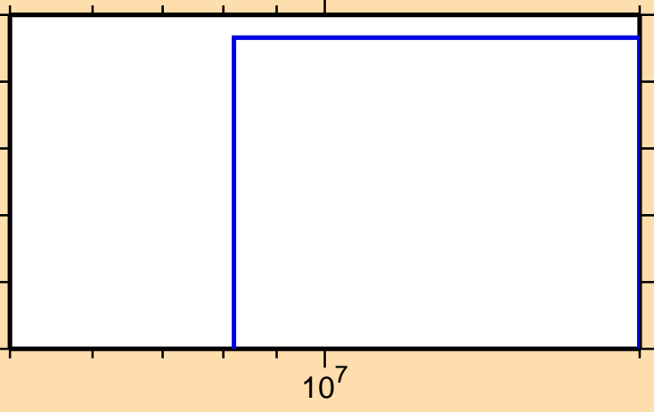
\sigma vs. E for ^{103}\text{Ru}(n,t)
