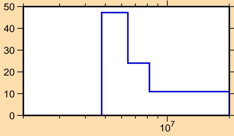
\Delta\sigma/\sigma vs. E for ^{103}\text{Ru}(n,2n)
