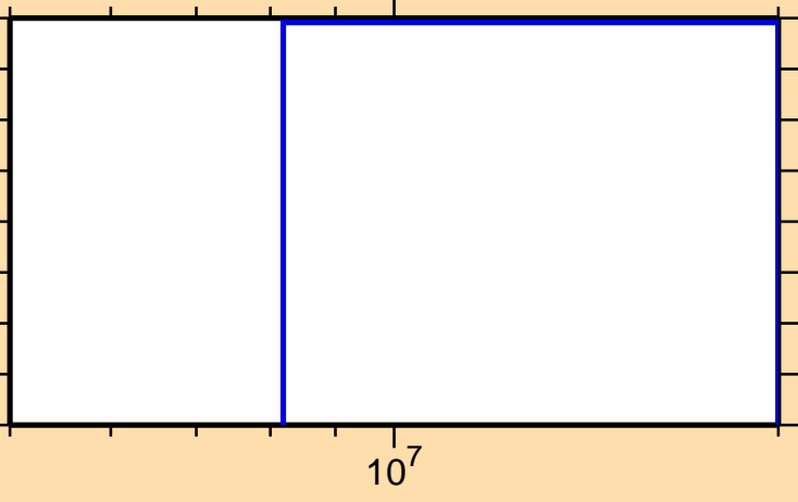
\sigma vs. E for ^{103}\text{Ru}(n,2np)
