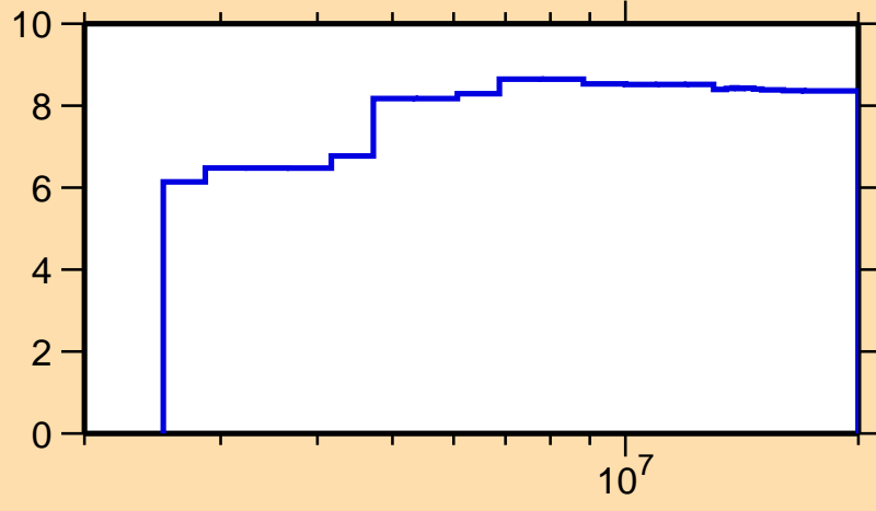
\Delta\sigma/\sigma vs. E for ^{104}\text{Ru}(n,n\text{onel.})
