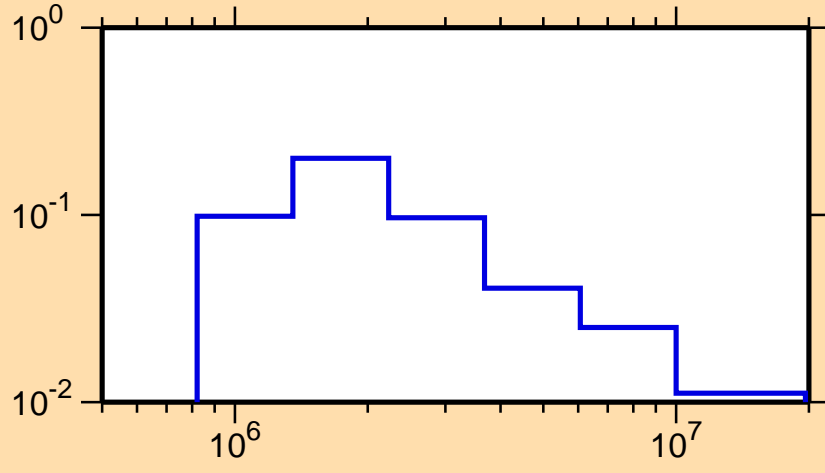
\sigma vs. E for ^{104}\text{Ru}(n,n_4)
