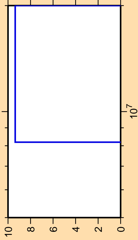
\Delta\sigma/\sigma vs. E for ^{104}\text{Ru}(n,nd)
