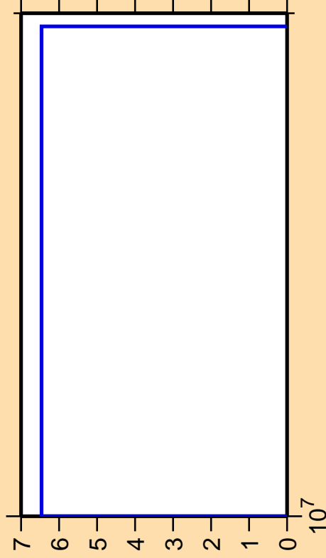
\Delta\sigma/\sigma vs. E for ^{105}\text{Ru}(n,nt)
