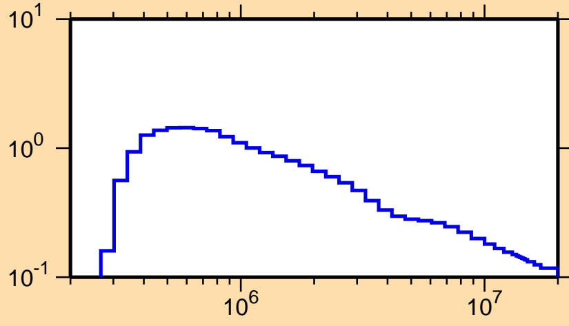
\sigma vs. E for ^{106}\text{Ru}(n,n_1)
