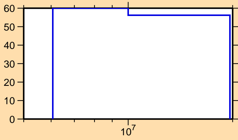
\Delta\sigma/\sigma vs. E for ^{106}\text{Ru}(n,p)
