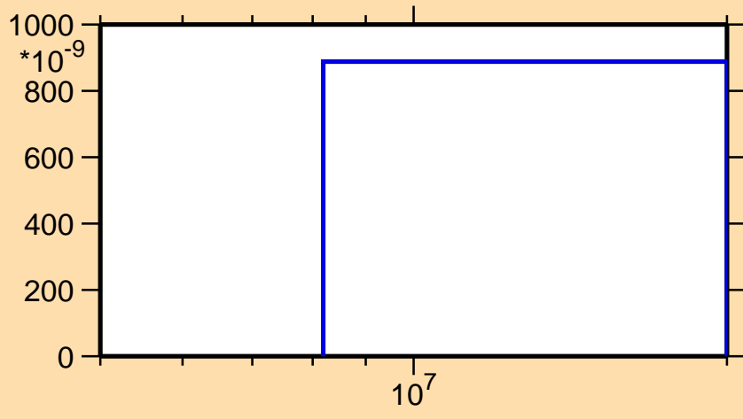
\sigma vs. E for ^{106}\text{Ru}(n,t)
