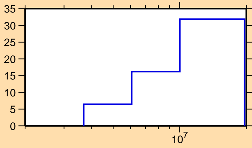
\Delta\sigma/\sigma vs. E for ^{107}\text{Ru}(n,ncont.)
