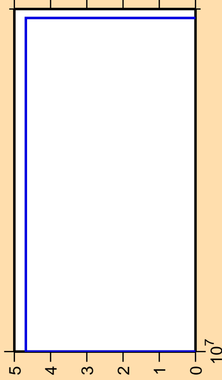
\Delta\sigma/\sigma vs. E for ^{107}\text{Ru}(n,2np)
