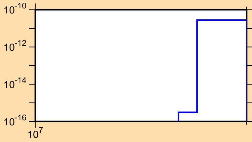
\sigma vs. E for ^{108}\text{Ru}(n,2n\alpha)
