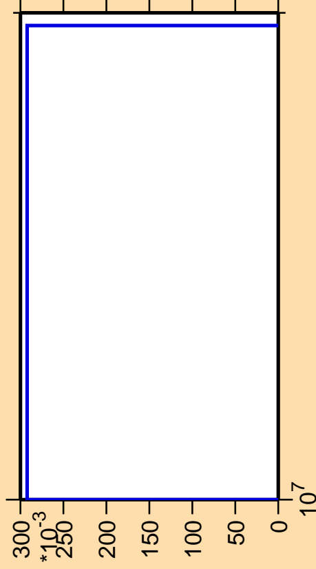
\Delta\sigma/\sigma vs. E for ^{108}\text{Ru}(n,2n\alpha)
