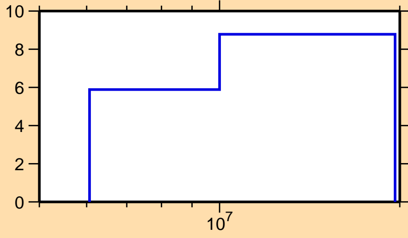
\Delta\sigma/\sigma vs. E for ^{108}\text{Ru}(n,2n)
