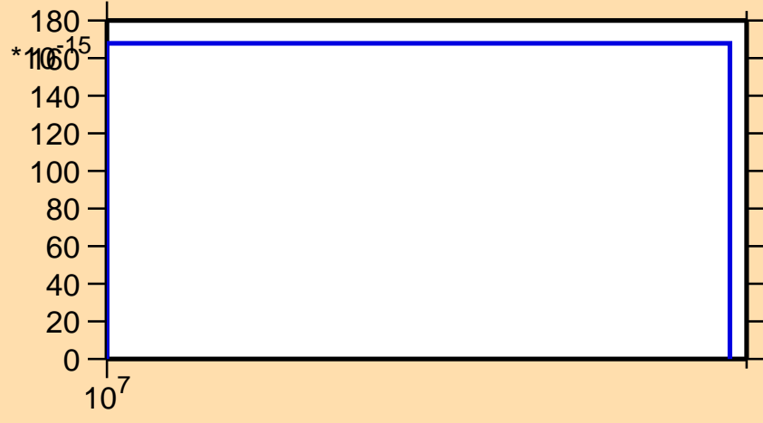
\sigma vs. E for ^{108}\text{Ru}(n,2n\alpha)
