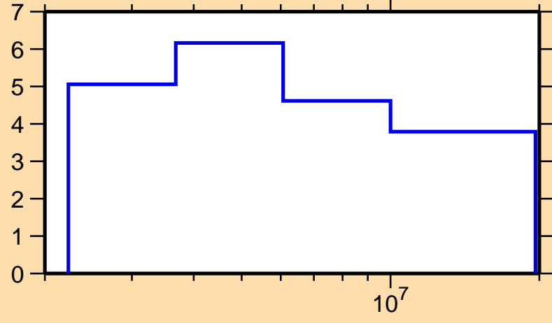
\Delta\sigma/\sigma vs. E for ^{108}\text{Ru}(n,n\text{onel.})
