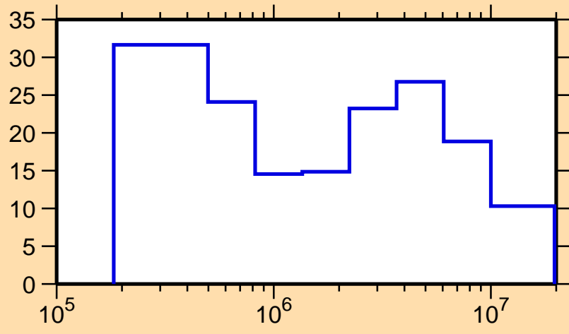
\Delta\sigma/\sigma vs. E for ^{108}\text{Ru}(n,n_1)
