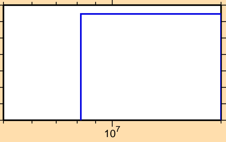
\sigma vs. E for ^{108}\text{Ru}(n,\text{nd})
