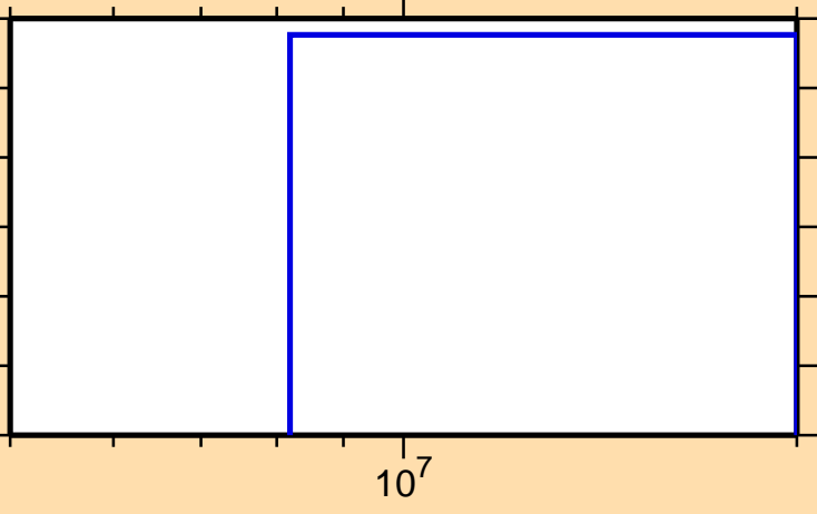
\sigma vs. E for ^{108}\text{Ru}(n,d)
