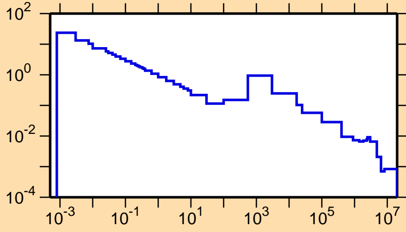
\sigma vs. E for ^{108}\text{Ru}(n,\gamma)
