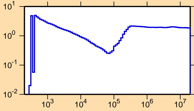
\sigma vs. E for ^{109}\text{Ru}(n,\text{nonel.})
