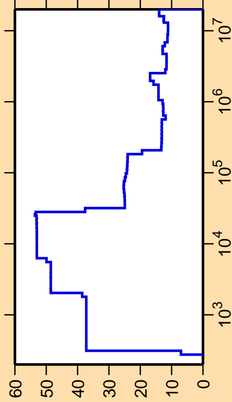
\Delta\sigma/\sigma vs. E for ^{109}\text{Ru}(n,\text{nonel.})
