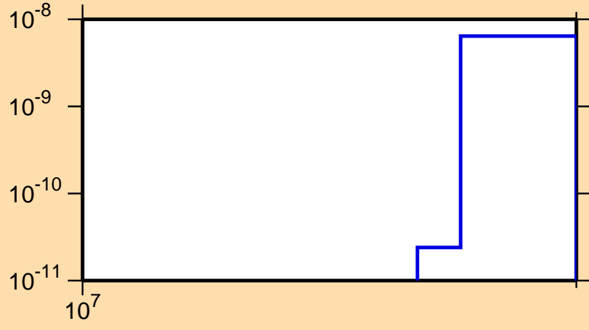
\sigma vs. E for ^{109}\text{Ru}(n,2n\alpha)
