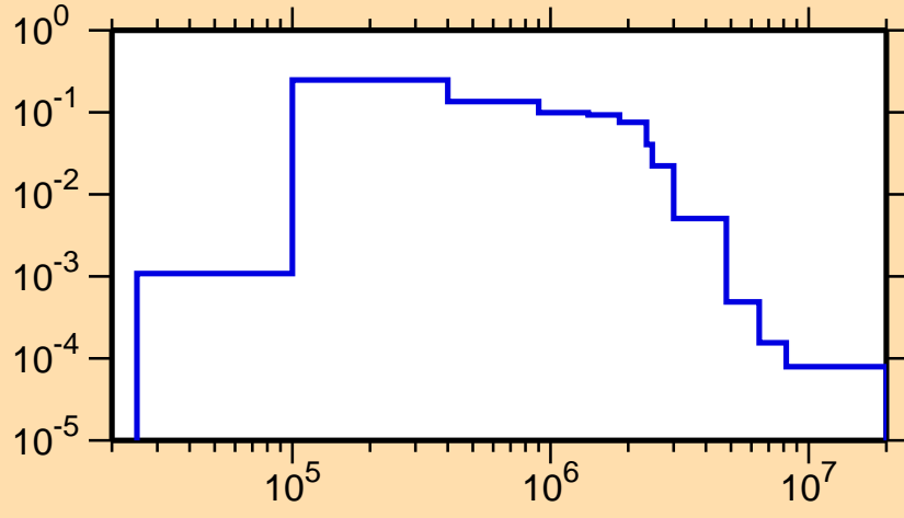
\sigma vs. E for ^{109}\text{Ru}(n,n_2)
