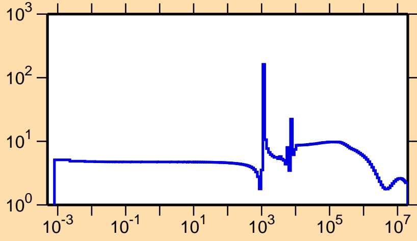
\sigma vs. E for ^{110}\text{Ru}(n,\text{el.})
