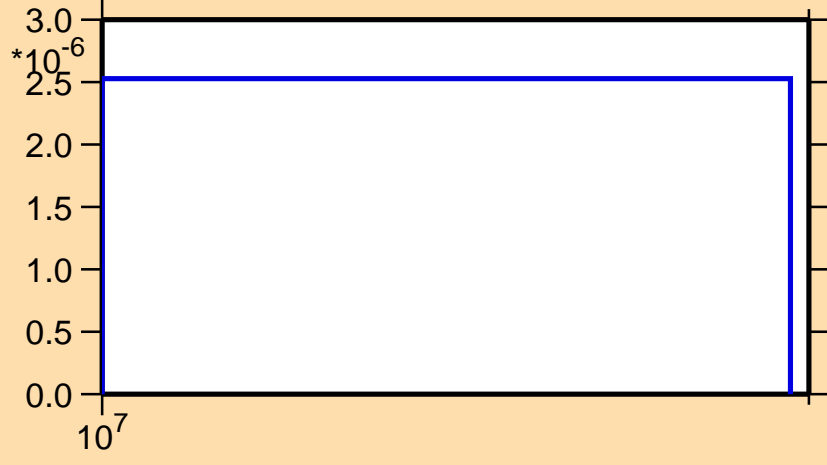
\sigma vs. E for ^{110}\text{Ru}(n,d)
