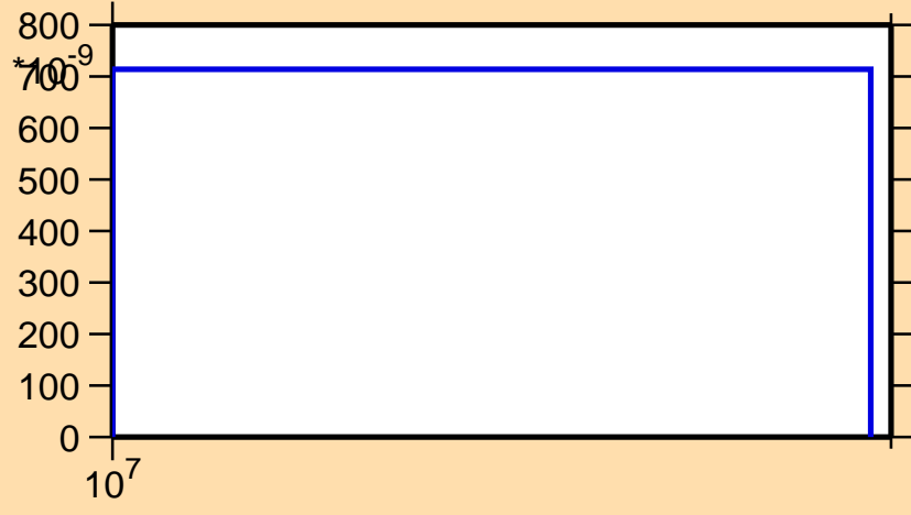
\sigma vs. E for ^{110}\text{Ru}(n,np)
