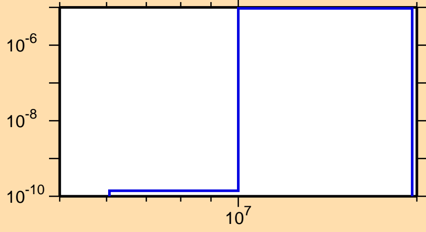
\sigma vs. E for ^{110}\text{Ru}(n,\alpha)
