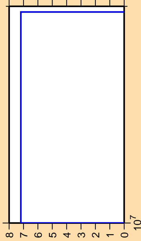
\Delta\sigma/\sigma vs. E for ^{110}\text{Ru}(n,nt)
