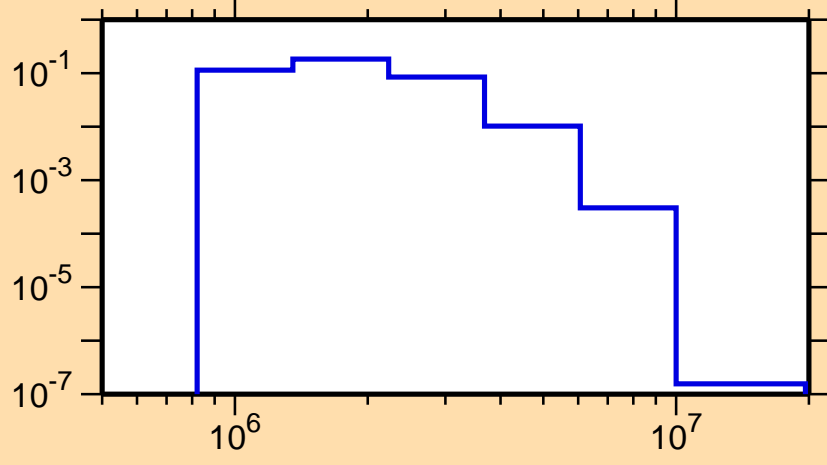
\sigma vs. E for ^{110}\text{Ru}(n,n_4)
