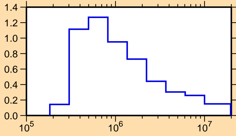
\sigma vs. E for ^{110}\text{Ru}(n,n_1)
