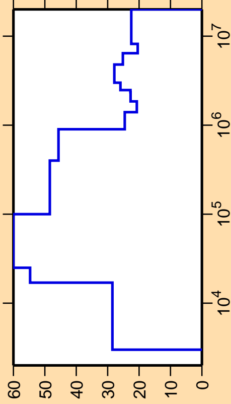
\Delta\sigma/\sigma vs. E for ^{110}\text{Ru}(n,\text{nonel.})
