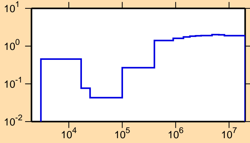
\sigma vs. E for ^{110}\text{Ru}(n,\text{nonel.})
