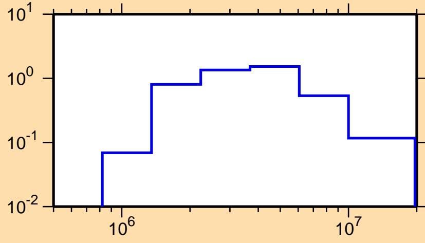
\sigma vs. E for ^{111}\text{Ru}(n,n\text{cont.})
