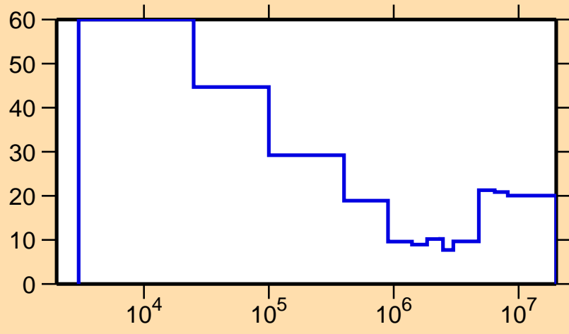
\Delta\sigma/\sigma vs. E for ^{111}\text{Ru}(n,\text{inel.})
