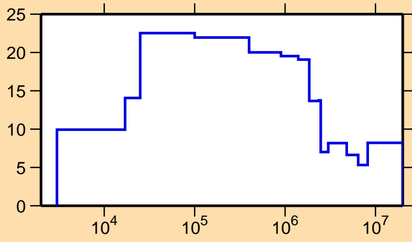
\Delta\sigma/\sigma vs. E for ^{111}\text{Ru}(n,\text{tot.})
