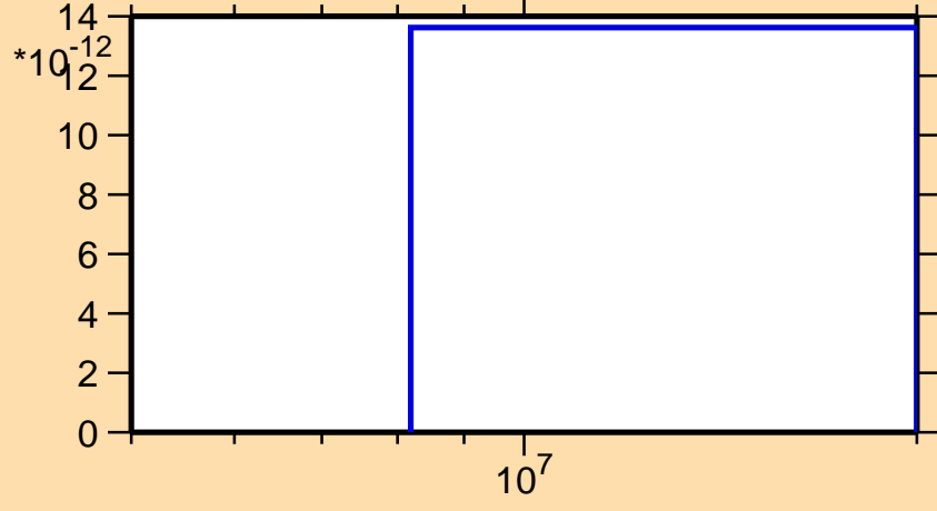
\sigma vs. E for ^{111}\text{Ru}(n,nt)
