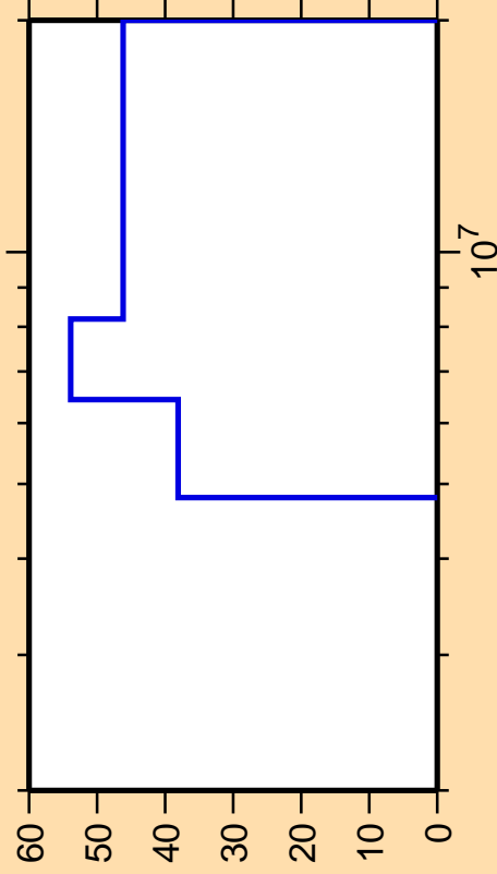
\Delta\sigma/\sigma vs. E for ^{111}\text{Ru}(n,n\text{cont.})
