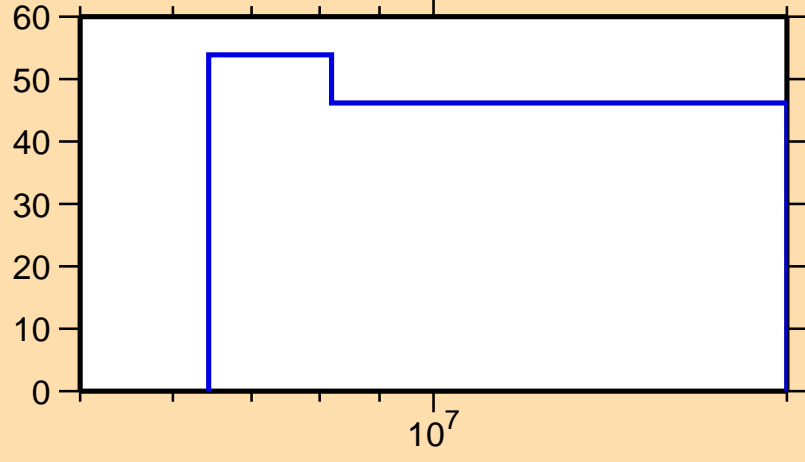
\Delta\sigma/\sigma vs. E for ^{111}\text{Ru}(n,n\text{cont.})
