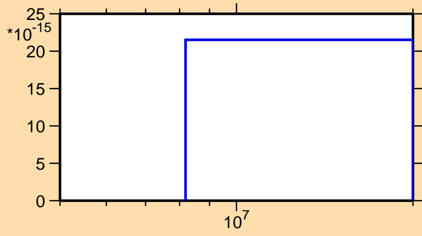
\sigma vs. E for ^{111}\text{Ru}(n,2np)
