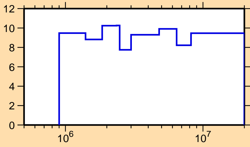
\Delta\sigma/\sigma vs. E for ^{111}\text{Ru}(n,\text{nonel.})
