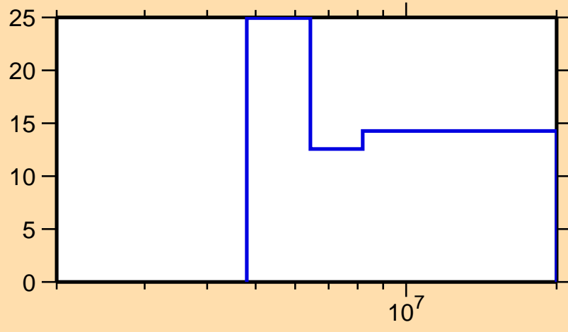
\Delta\sigma/\sigma vs. E for ^{111}\text{Ru}(n,2n)
