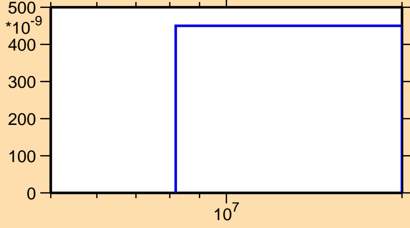
\sigma vs. E for ^{111}\text{Ru}(n,n\alpha)
