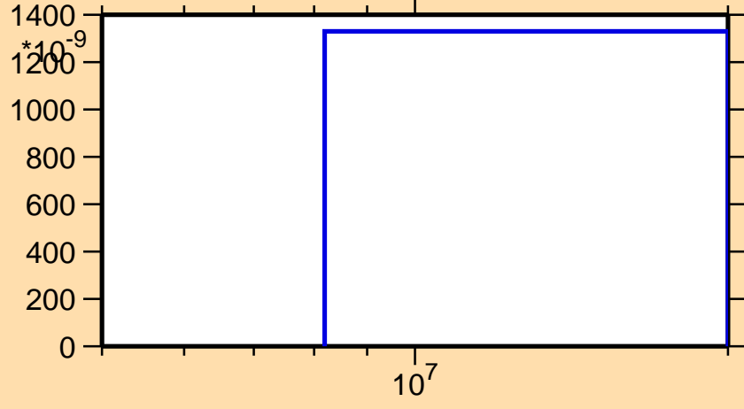
\sigma vs. E for ^{111}\text{Ru}(n,t)
