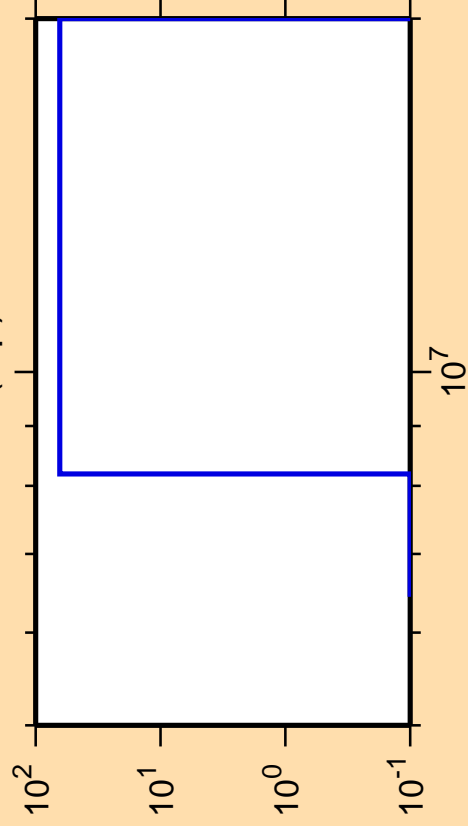
\Delta\sigma/\sigma vs. E for ^{111}\text{Ru}(n,p)
