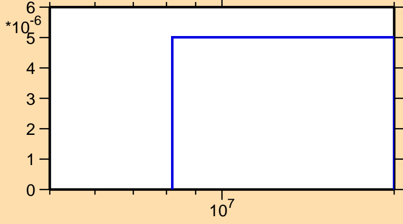
\sigma vs. E for ^{111}\text{Ru}(n,d)
