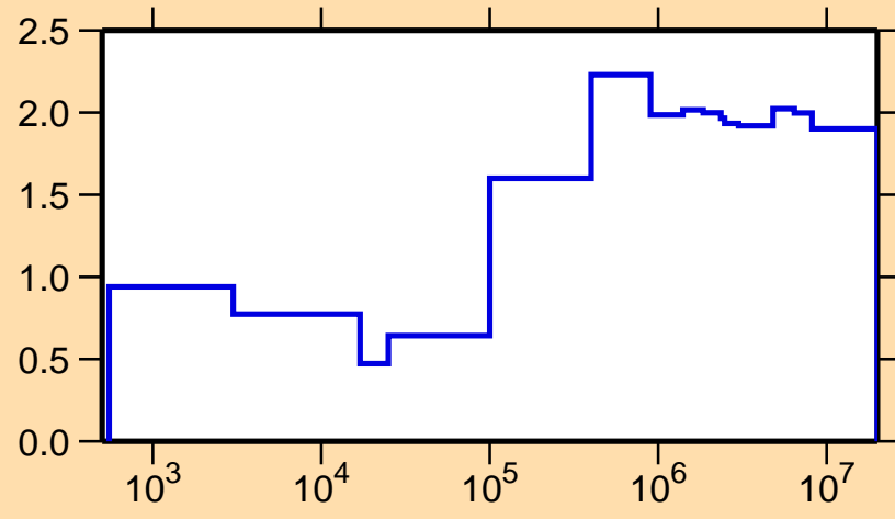
\sigma vs. E for ^{111}\text{Ru}(n,\text{nonel.})
