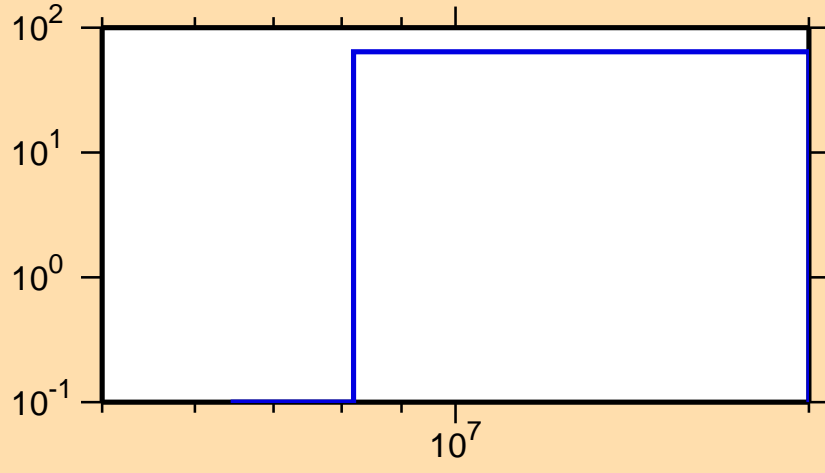
\Delta\sigma/\sigma vs. E for ^{111}\text{Ru}(n,p)
