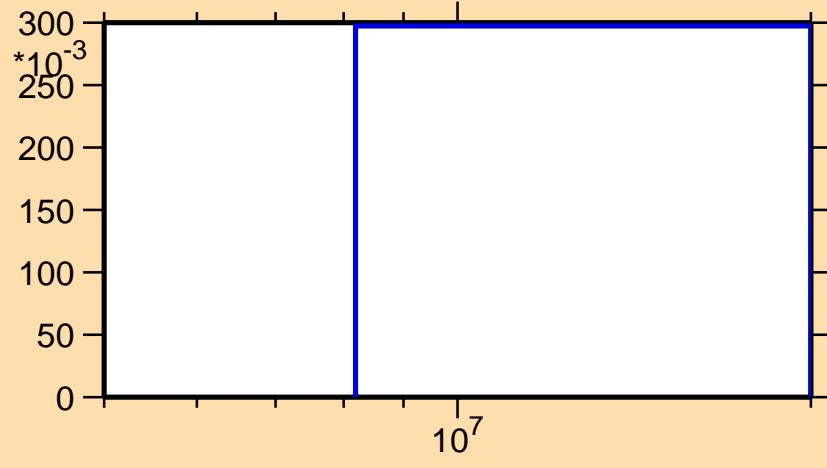
\sigma vs. E for ^{111}\text{Ru}(n,3n)
