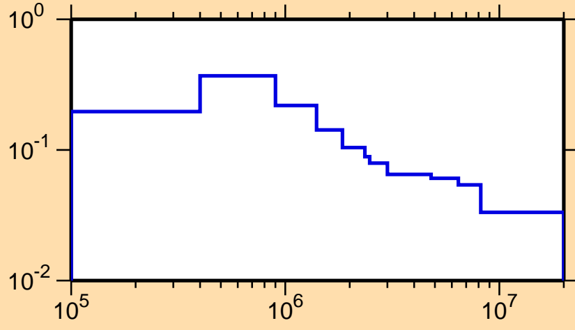
\sigma vs. E for ^{111}\text{Ru}(n,n_4)
