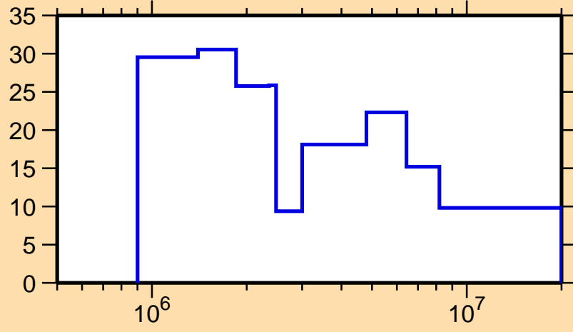
\Delta\sigma/\sigma vs. E for ^{111}\text{Ru}(n,\text{el.})
