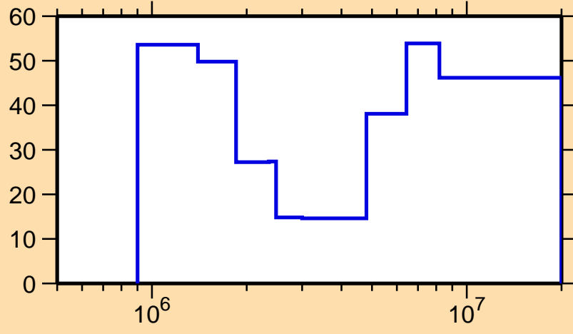
\Delta\sigma/\sigma vs. E for ^{111}\text{Ru}(n,n\text{cont.})
