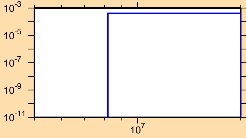
\sigma vs. E for ^{111}\text{Ru}(n,p)
