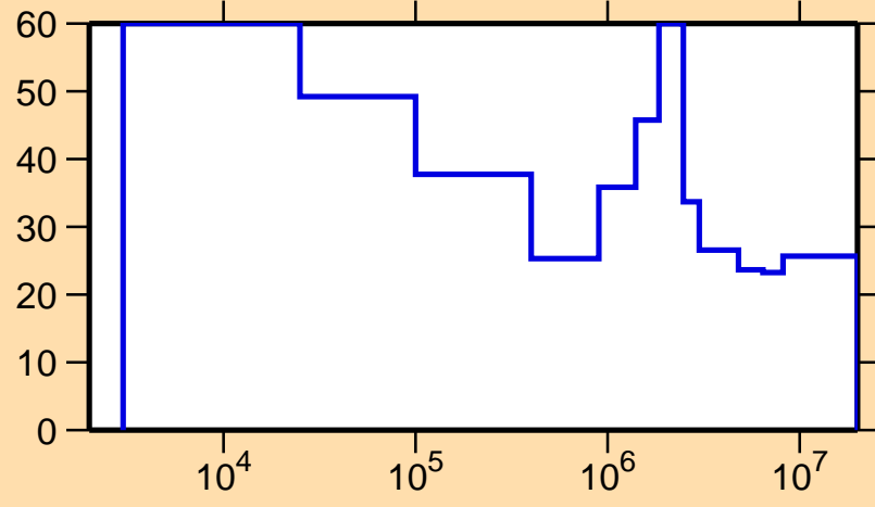
\Delta\sigma/\sigma vs. E for ^{111}\text{Ru}(n,n_1)
