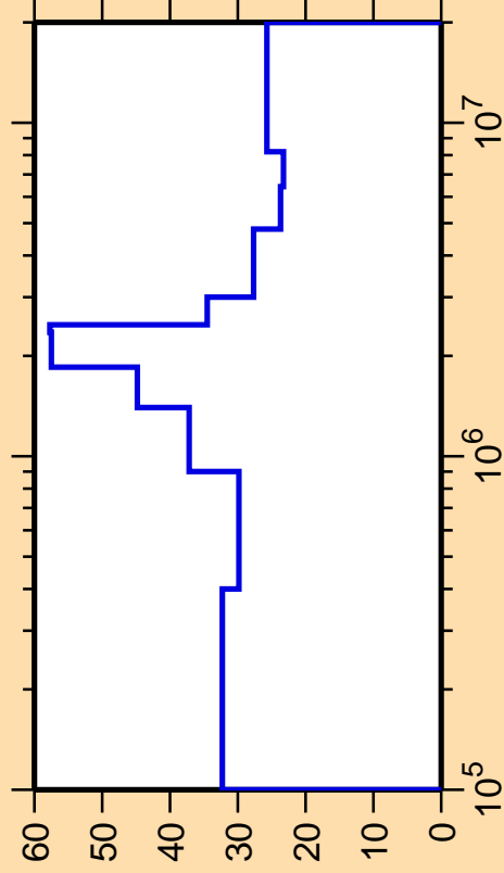
\Delta\sigma/\sigma vs. E for ^{111}\text{Ru}(n,n_4)
