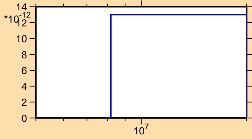
\sigma vs. E for ^{111}\text{Ru}(n,2n\alpha)
