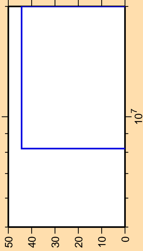
\Delta\sigma/\sigma vs. E for ^{111}\text{Ru}(n,2n\alpha)
