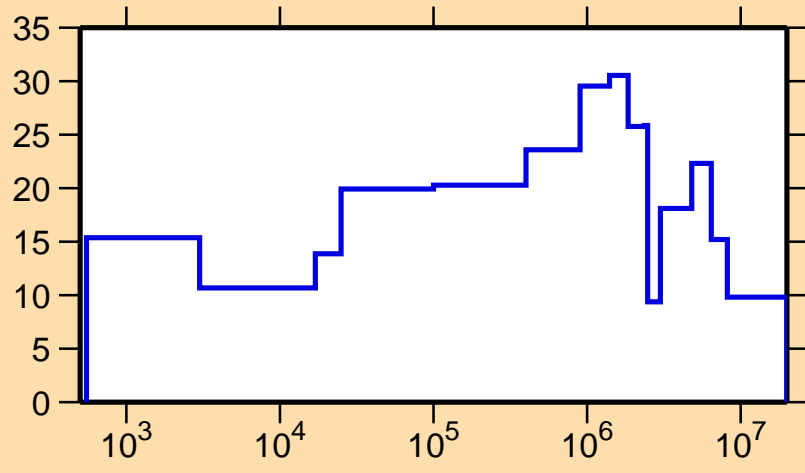
\Delta\sigma/\sigma vs. E for ^{111}\text{Ru}(n,\text{el.})
