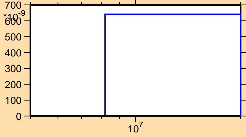
\sigma vs. E for ^{111}\text{Ru}(n,np)
