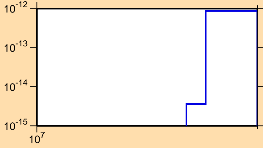
\sigma vs. E for ^{112}\text{Ru}(n,2n\alpha)
