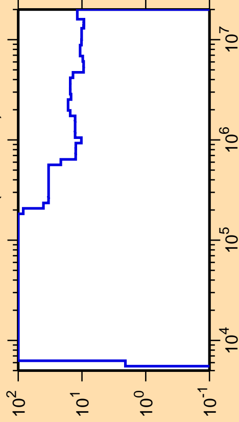
\Delta\sigma/\sigma vs. E for ^{112}\text{Ru}(n,\text{nonel.})
