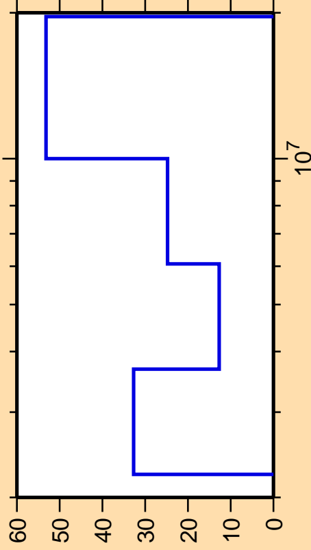
\Delta\sigma/\sigma vs. E for ^{112}\text{Ru}(n,n\text{cont.})
