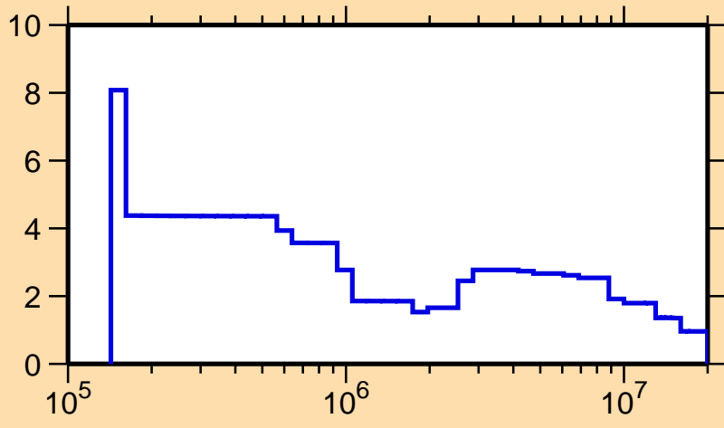
\Delta\sigma/\sigma vs. E for ^{30}\text{S}(n,\text{tot.})
