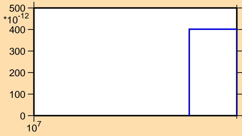
\sigma vs. E for ^{30}\text{S} (mt 34)
