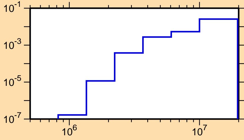
\sigma vs. E for ^{30}\text{S}(n,\text{He}3)
