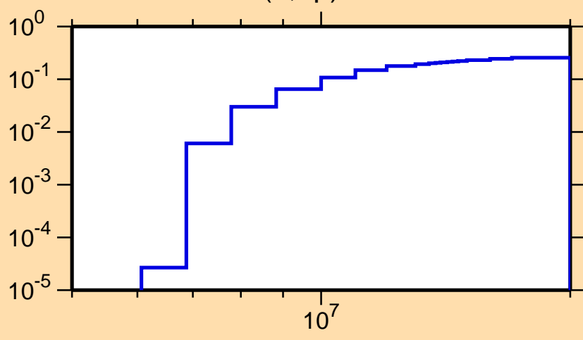
\sigma vs. E for ^{31}\text{S}(n,np)
