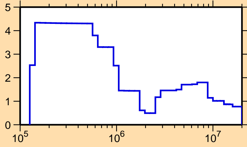
\Delta\sigma/\sigma vs. E for ^{31}\text{S}(n,\text{tot.})
