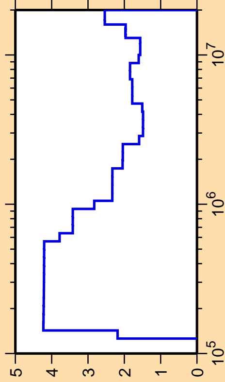
\Delta\sigma/\sigma vs. E for ^{31}\text{S}(n,\text{nonel.})
