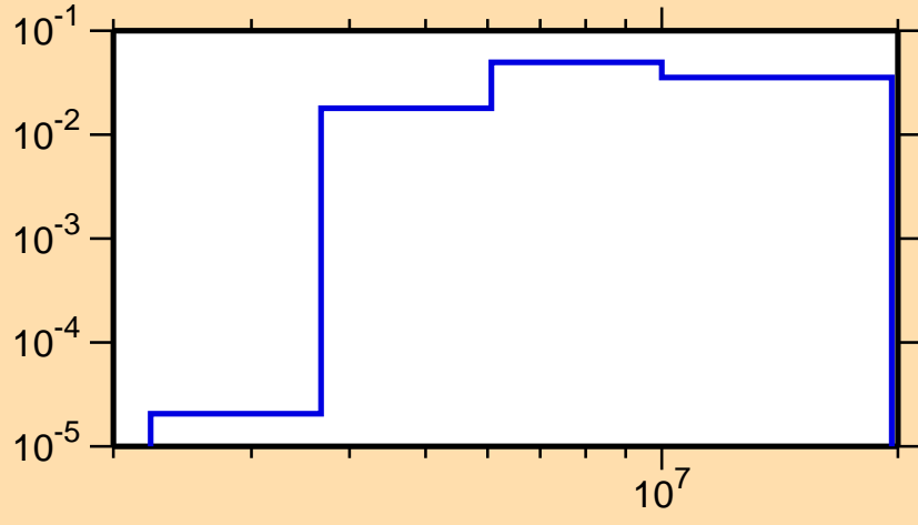
\sigma vs. E for ^{31}\text{S}(n,n\text{cont.})
