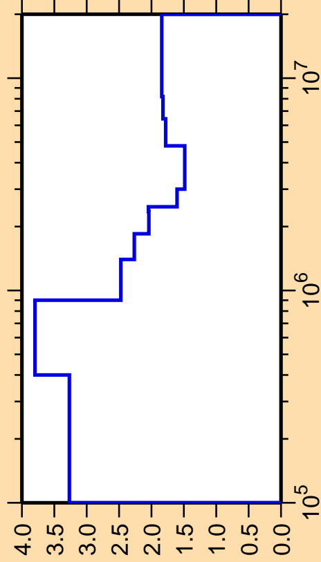
\Delta\sigma/\sigma vs. E for ^{31}\text{S}(n,\text{nonel.})
