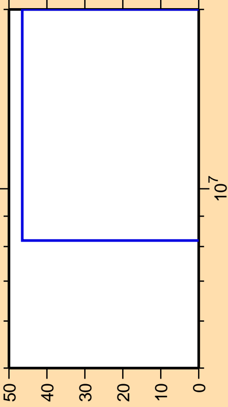
\Delta\sigma/\sigma vs. E for ^{31}\text{S}(n,\text{pd})
