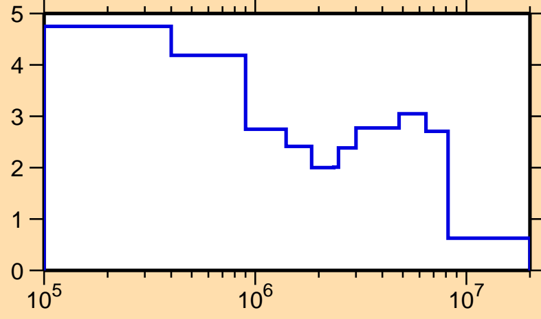
\Delta\sigma/\sigma vs. E for ^{31}\text{S}(n,el.)
