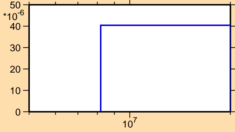
\sigma vs. E for ^{31}\text{S}(n,\text{pt})
