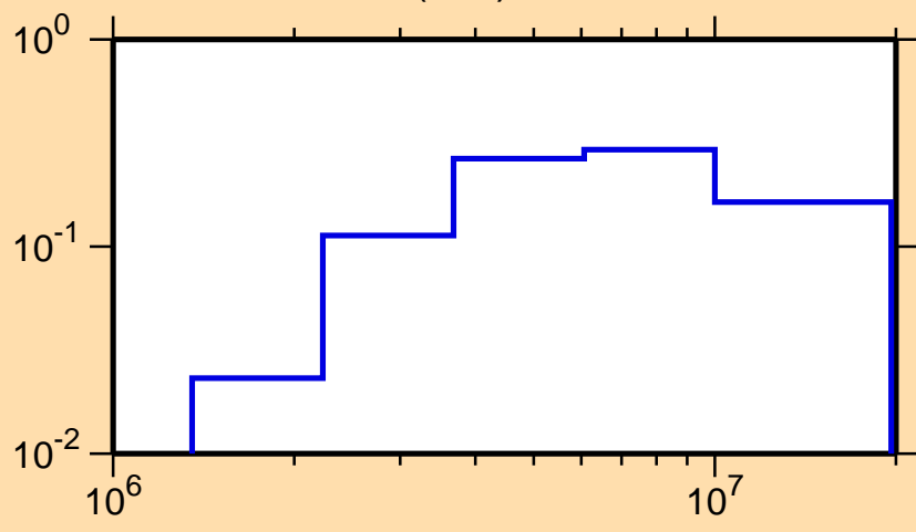
\sigma vs. E for ^{32}\text{S}(n,\alpha)
