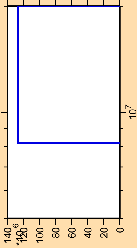
\Delta\sigma/\sigma vs. E for ^{32}\text{S}(n,nd)
