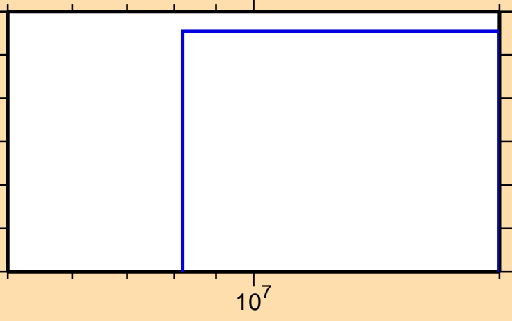
\sigma vs. E for ^{32}\text{S}(n,\text{He}3)
