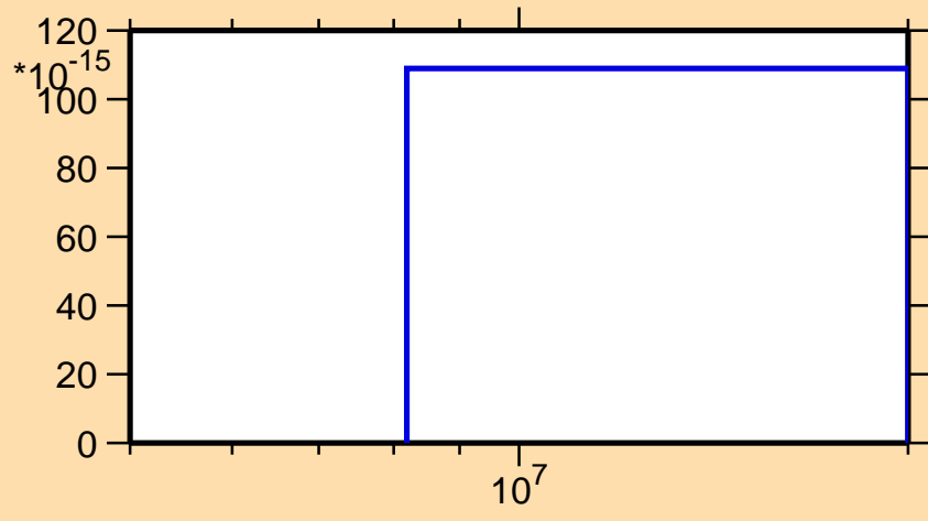
\sigma vs. E for ^{32}\text{S}(\text{mt117})
