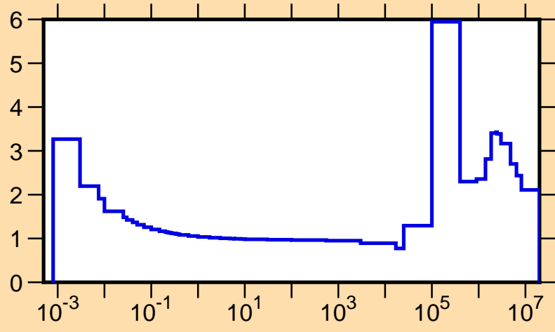
\sigma vs. E for ^{32}\text{S}(n,\text{tot.})
