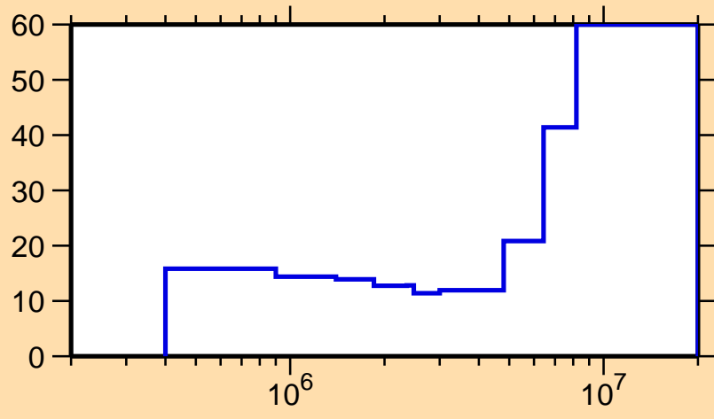
\Delta\sigma/\sigma vs. E for ^{33}\text{S}(n,n_1)
