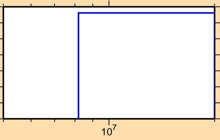
\sigma vs. E for ^{33}\text{S}(n,nd)
