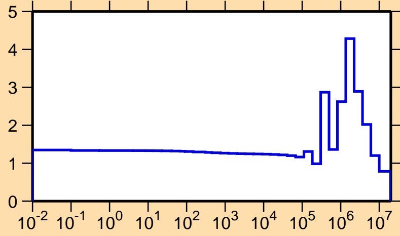
\sigma vs. E for ^{34}\text{S}(n,\text{el.})
