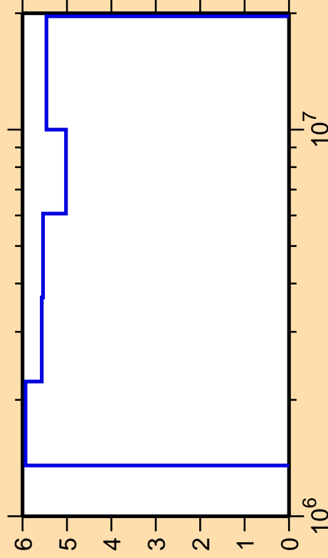
\Delta\sigma/\sigma vs. E for ^{34}\text{S}(n,\text{nonel.})
