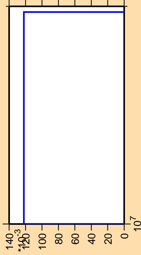
\Delta\sigma/\sigma vs. E for ^{34}\text{S}(n,nd)
