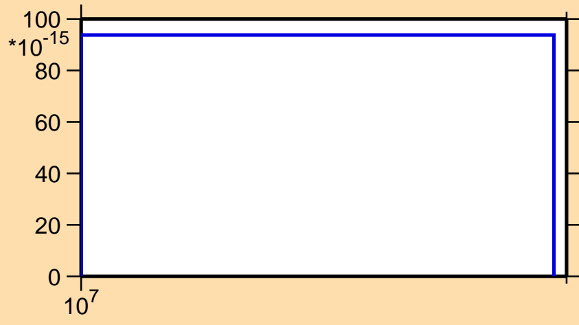
\sigma vs. E for ^{34}\text{S}(n,nd)
