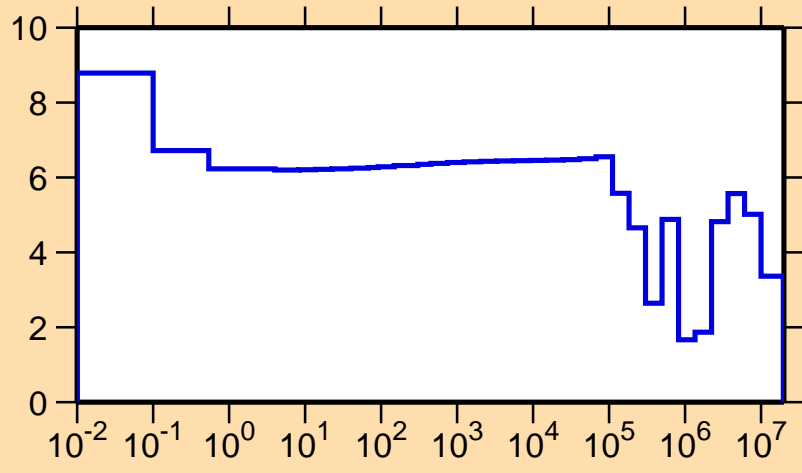
\Delta\sigma/\sigma vs. E for ^{34}\text{S}(n,\text{tot.})
