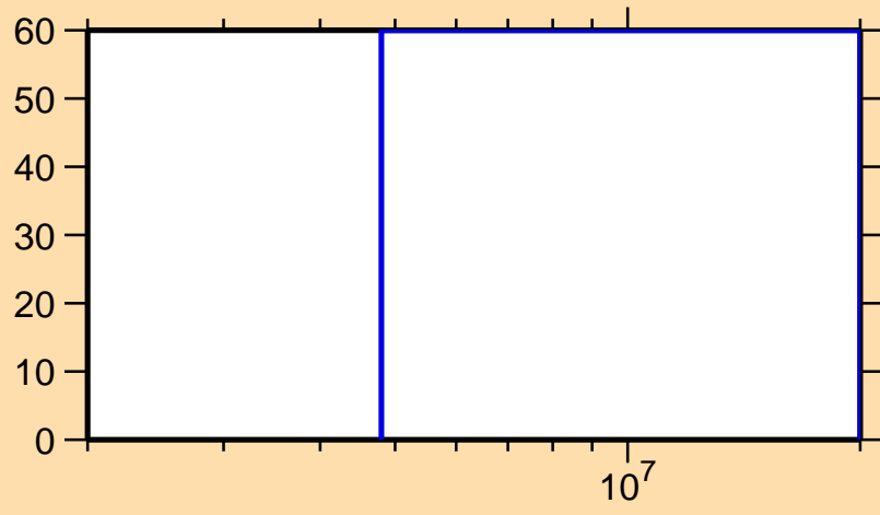
\Delta\sigma/\sigma vs. E for ^{34}\text{S}(n,\gamma)
