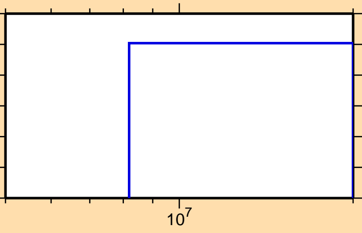
\sigma vs. E for ^{34}\text{S}(n,d)
