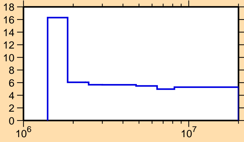
\Delta\sigma/\sigma vs. E for ^{34}\text{S}(n,\text{nonel.})
