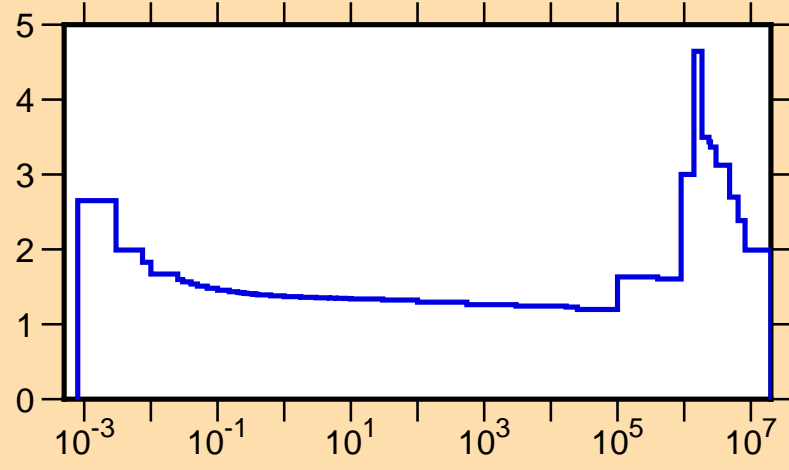
\sigma vs. E for ^{34}\text{S}(n,\text{tot.})
