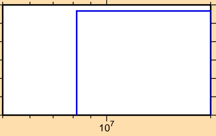
\sigma vs. E for ^{34}\text{S}(n,\text{He}3)
