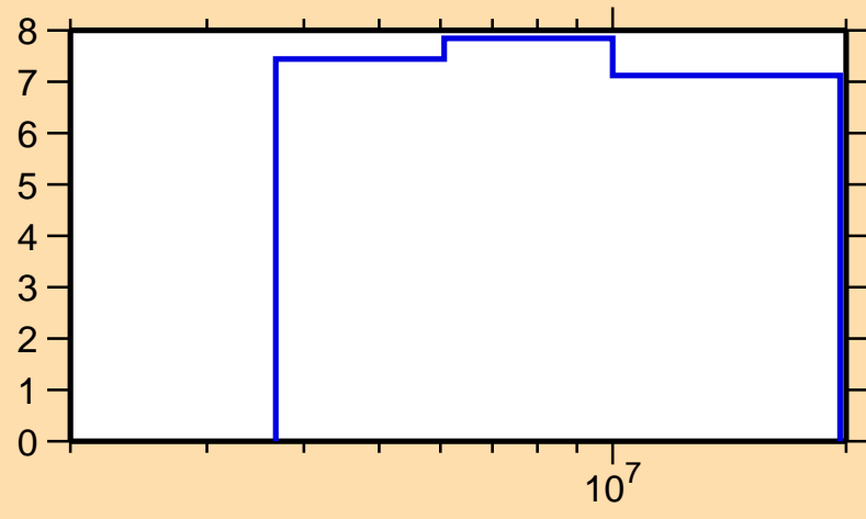
\Delta\sigma/\sigma vs. E for ^{35}\text{S}(n,n\text{onel.})
