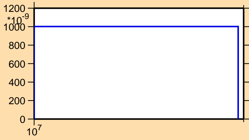
\sigma vs. E for ^{35}\text{S}(n,nd)
