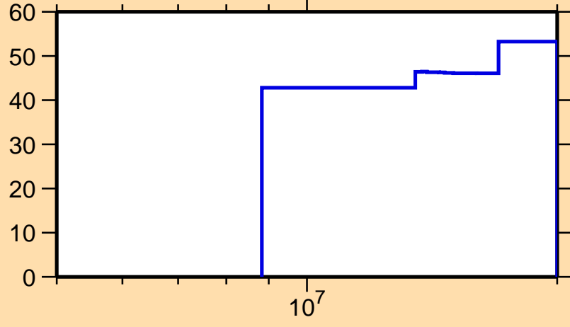
\Delta\sigma/\sigma vs. E for ^{36}\text{S}(n,p)
