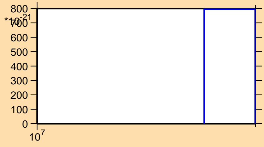
\sigma vs. E for ^{36}\text{S}(n,\text{nd})
