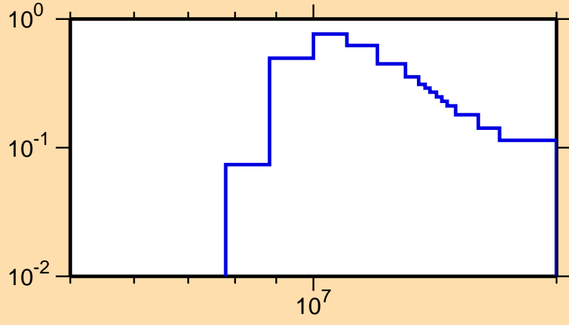
\sigma vs. E for ^{36}\text{S}(n,n\text{cont.})
