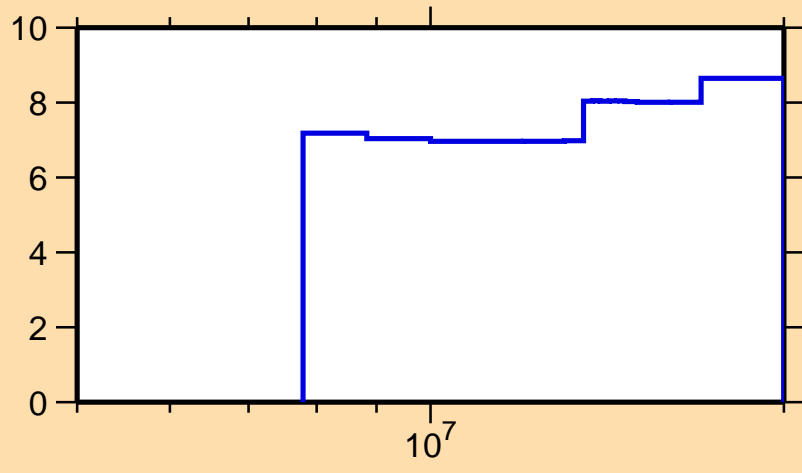
\Delta\sigma/\sigma vs. E for ^{36}\text{S}(n,n\text{onel.})
