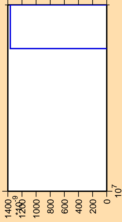
\Delta\sigma/\sigma vs. E for ^{36}\text{S}(n,\text{nd})
