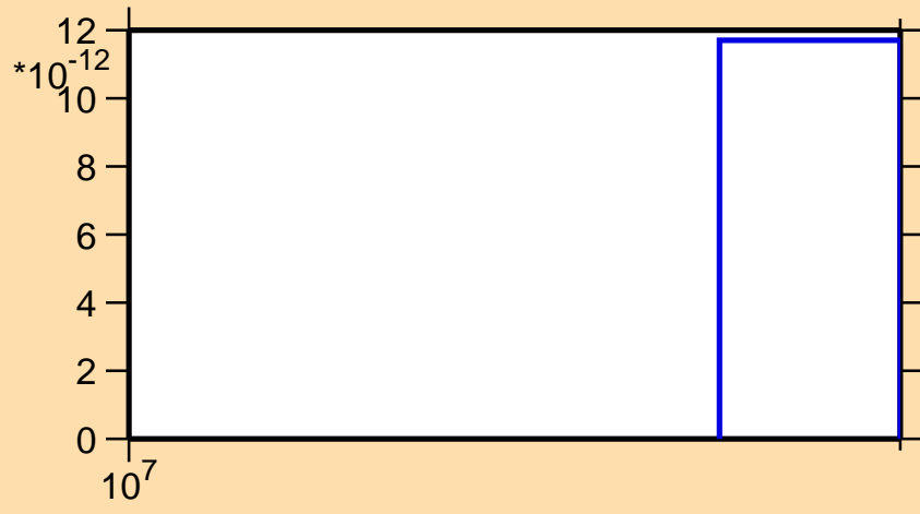
\sigma vs. E for ^{36}\text{S}(n,nt)
