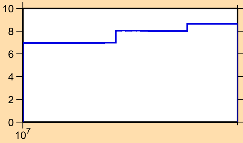
\Delta\sigma/\sigma vs. E for ^{36}\text{S}(n,\text{nonel.})
