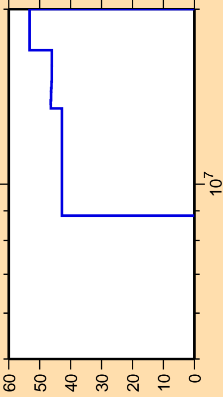
\Delta\sigma/\sigma vs. E for ^{36}\text{S}(n,p)
