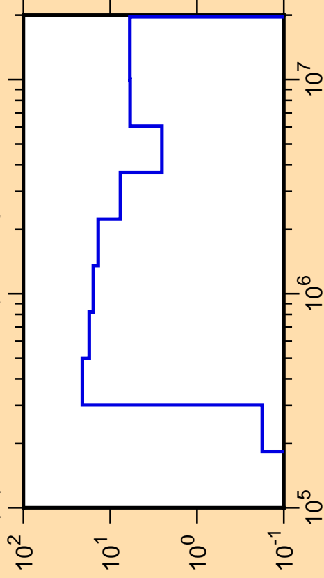
\Delta\mu/\mu vs. E for ^{36}\text{S} (mt251)
