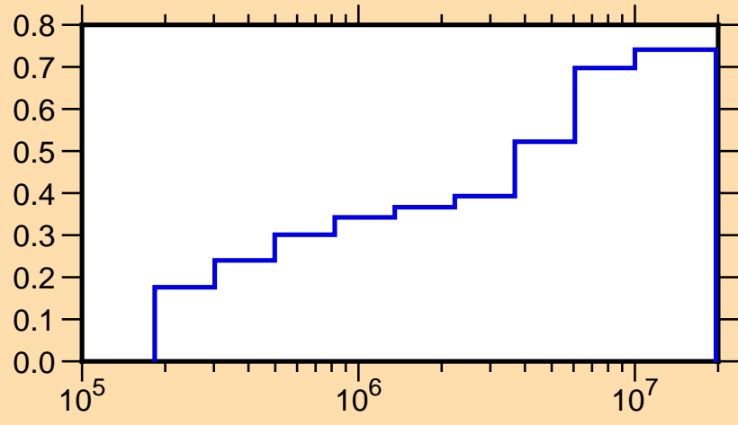
\mu vs. E for ^{36}\text{S} (mt251)
