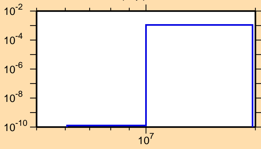
\sigma vs. E for ^{36}\text{S}(n,p)
