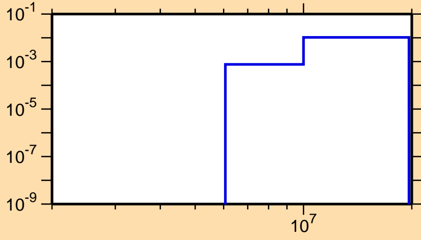
\sigma vs. E for ^{36}\text{S}(n,\alpha)
