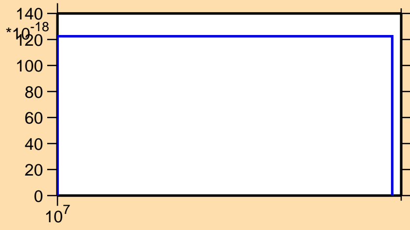
\sigma vs. E for ^{36}\text{S}(n,2n\alpha)
