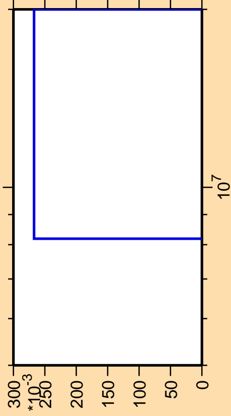
\Delta\sigma/\sigma vs. E for ^{36}\text{S}(n,nt)
