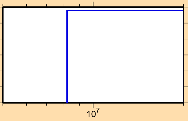
\sigma vs. E for ^{36}\text{S}(n,d)
