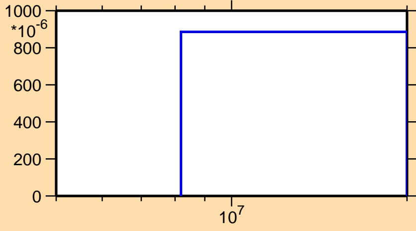
\sigma vs. E for ^{36}\text{S}(n,p)
