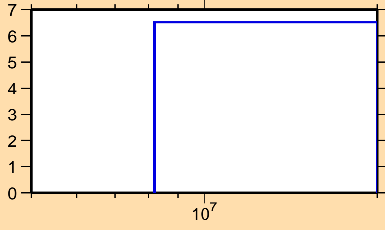
\Delta\sigma/\sigma vs. E for ^{36}\text{S}(n,el.)
