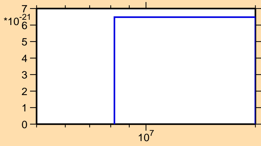
\sigma vs. E for ^{36}\text{S}(n,nd)
