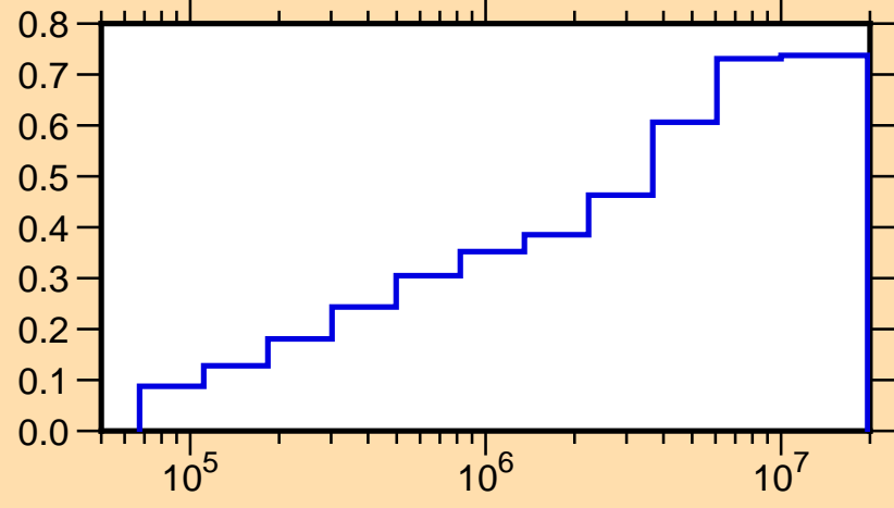
\mu vs. E for ^{37}\text{S}(\text{mt251})
