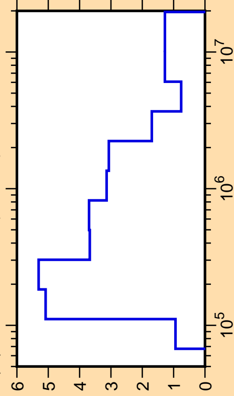
\Delta\mu/\mu vs. E for ^{37}\text{S}(\text{mt251})
