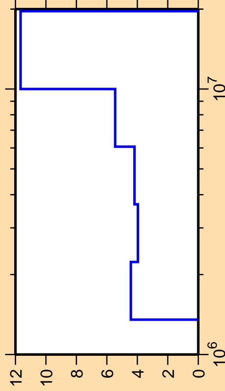
\Delta\sigma/\sigma vs. E for ^{37}\text{S}(n,n_2)
