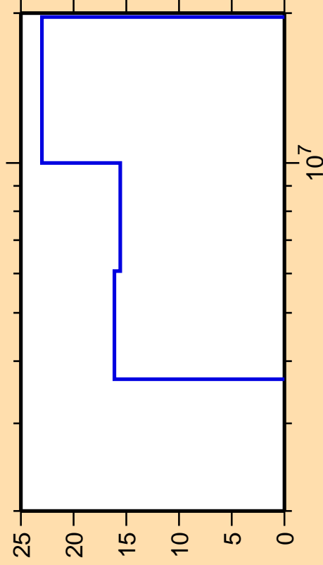
\Delta\sigma/\sigma vs. E for ^{37}\text{S}(n,\text{ncont.})
