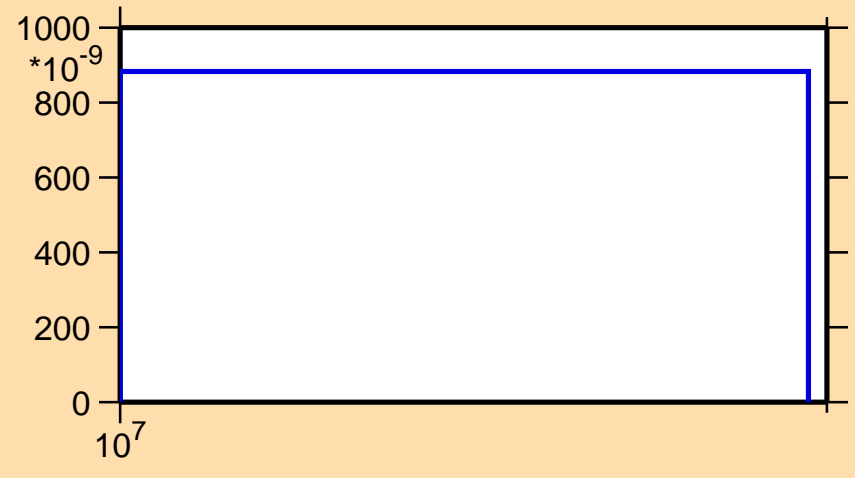
\sigma vs. E for ^{37}\text{S}(n,nd)
