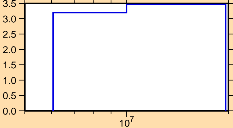
\Delta\sigma/\sigma vs. E for ^{37}\text{S}(n,2n)
