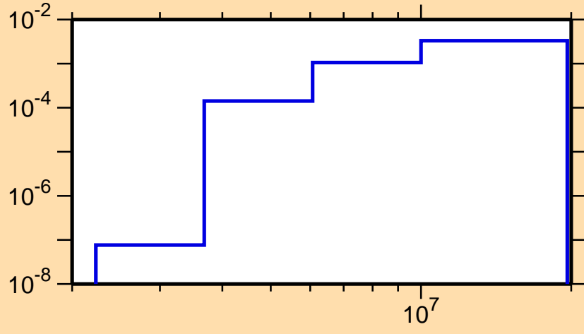
\sigma vs. E for ^{37}\text{S}(n,\alpha)
