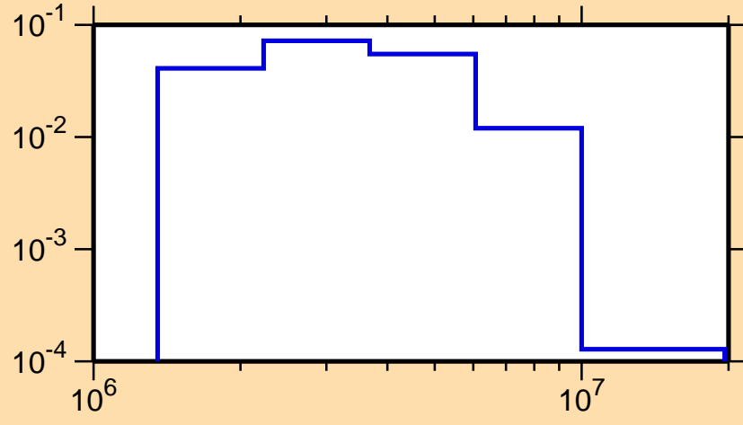
\sigma vs. E for ^{37}\text{S}(n,n_2)
