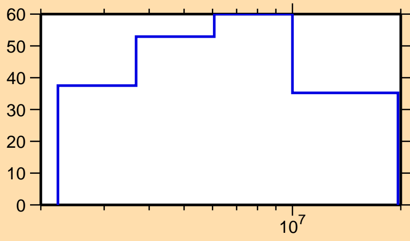
\Delta\sigma/\sigma vs. E for ^{37}\text{S}(n,\gamma)
