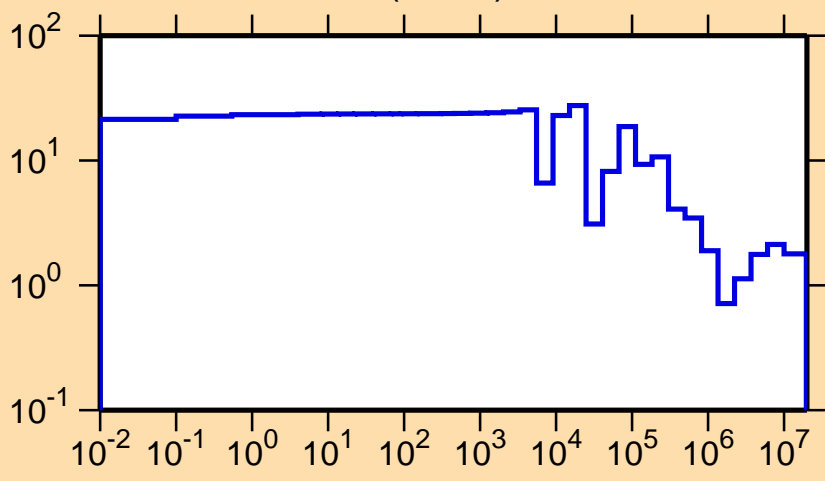
\Delta\sigma/\sigma vs. E for ^{37}\text{S}(n,\text{tot.})
