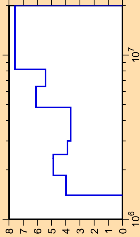
\Delta\sigma/\sigma vs. E for ^{37}\text{S}(n,n_2)
