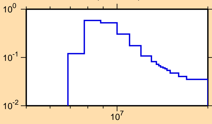
\sigma vs. E for ^{38}\text{S}(n,n\text{cont.})
