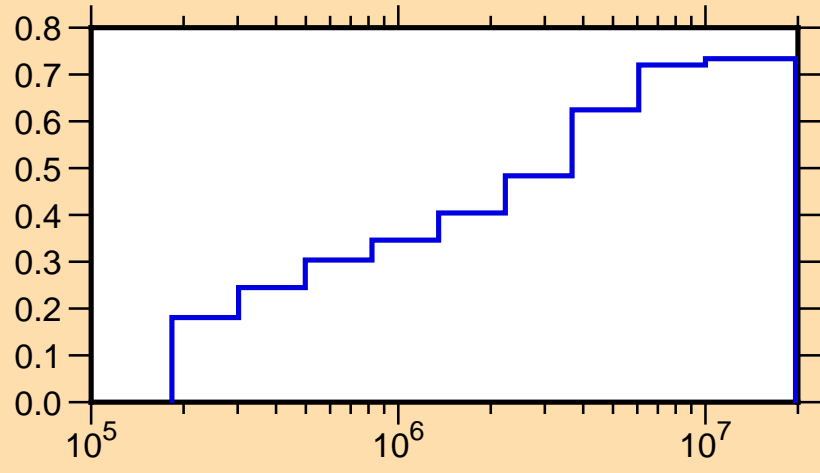
\mu vs. E for ^{38}\text{S} (mt251)
