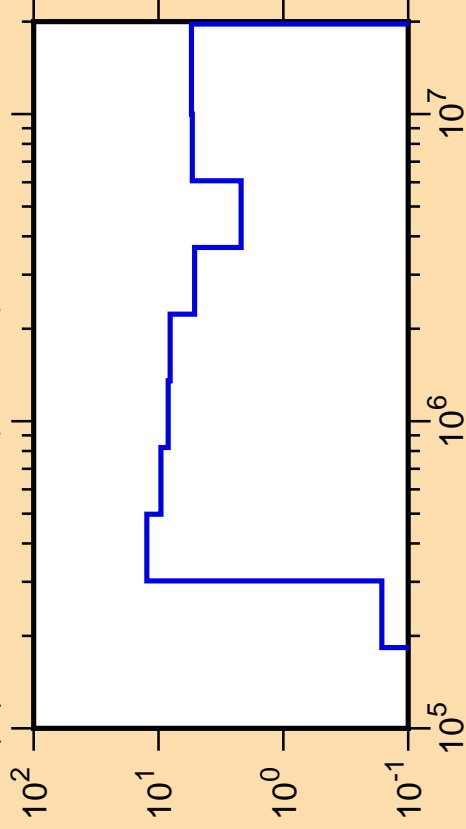
\Delta\mu/\mu vs. E for ^{38}\text{S} (mt251)
