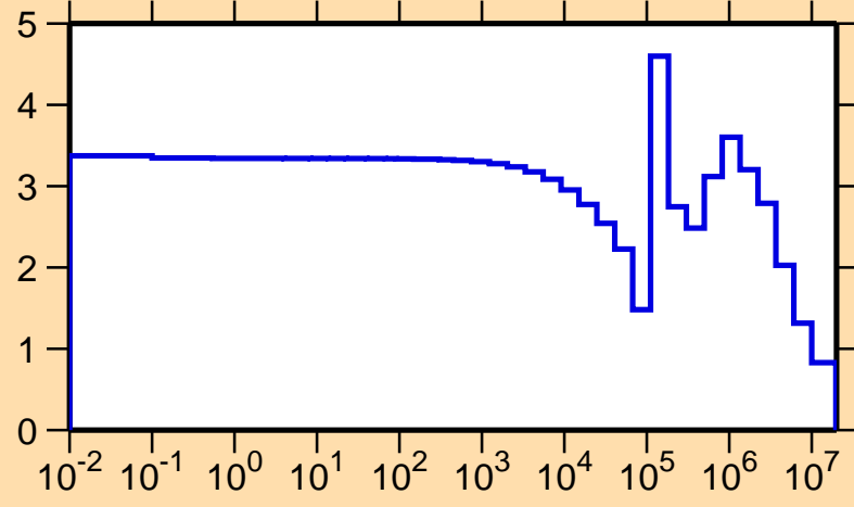
\sigma vs. E for ^{38}\text{S}(n,\text{el.})
