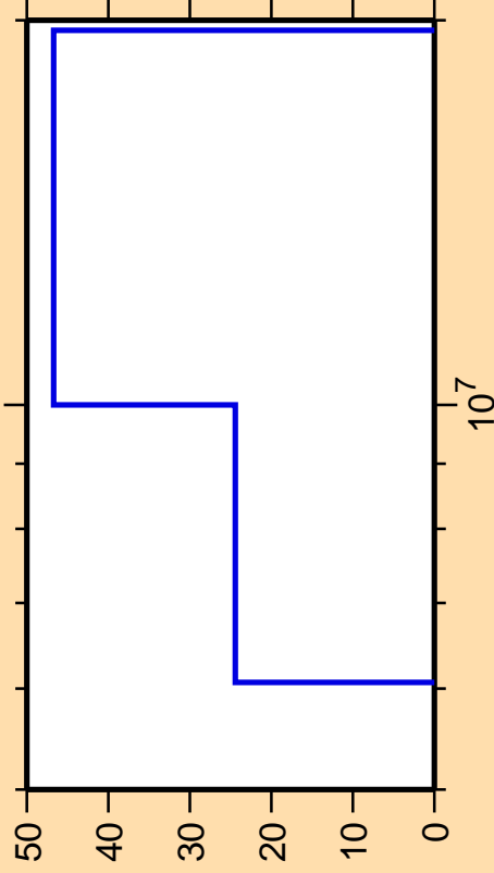
\Delta\sigma/\sigma vs. E for ^{38}\text{S}(n,n_1)
