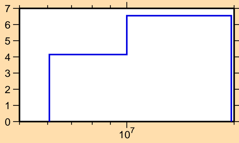
\Delta\sigma/\sigma vs. E for ^{38}\text{S}(n,n\text{onel.})
