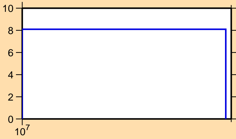
\Delta\sigma/\sigma vs. E for ^{38}\text{S}(n,el.)
