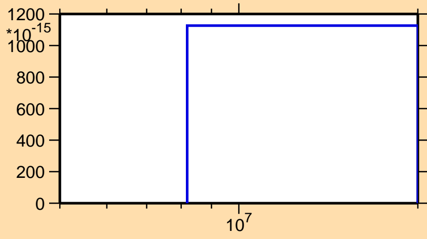
\sigma vs. E for ^{38}\text{S}(n,2n\alpha)
