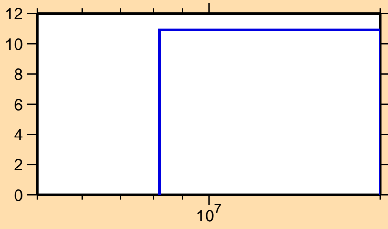
\Delta\sigma/\sigma vs. E for ^{38}\text{S}(n,2n)
