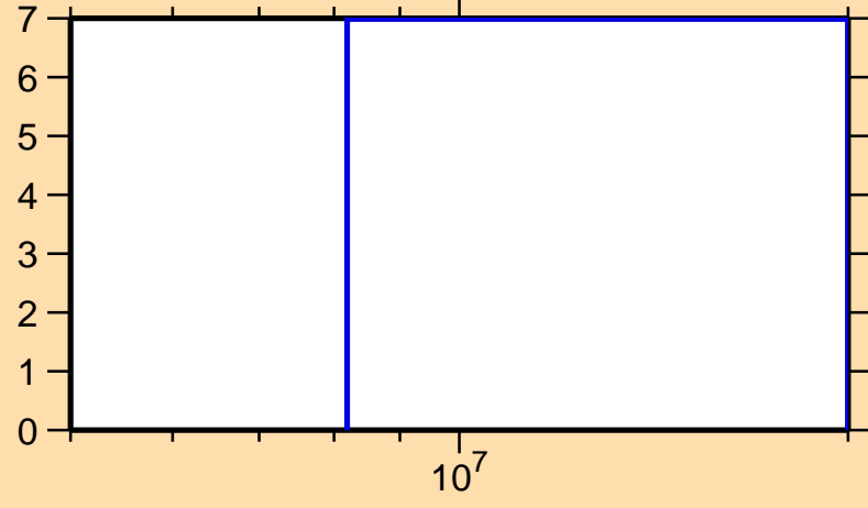
\Delta\sigma/\sigma vs. E for ^{38}\text{S}(n,el.)
