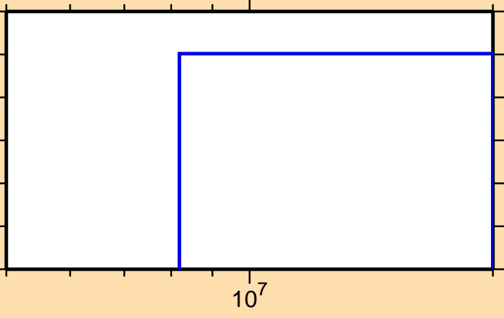
\sigma vs. E for ^{38}\text{S}(n,d)
