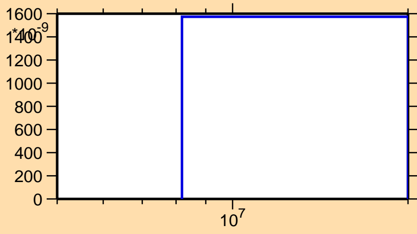
\sigma vs. E for ^{38}\text{S}(n,t)
