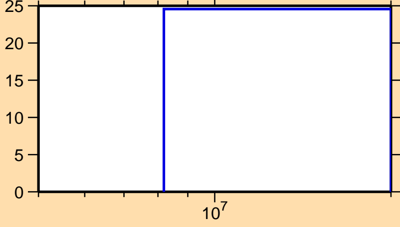
\Delta\sigma/\sigma vs. E for ^{38}\text{S}(n,ncont.)
