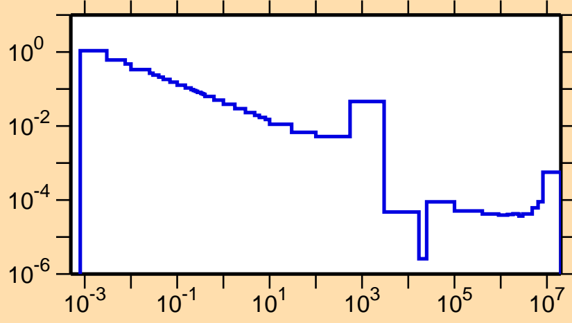
\sigma vs. E for ^{39}\text{S}(n,\gamma)
