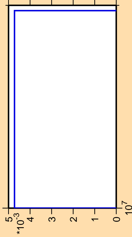
\Delta\sigma/\sigma vs. E for ^{40}\text{S}(n,nt)
