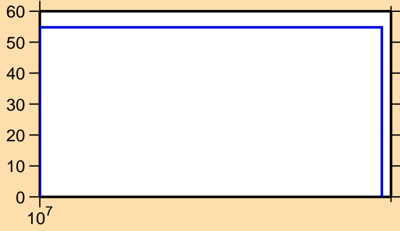
\Delta\sigma/\sigma vs. E for ^{40}\text{S}(n,n\text{cont.})
